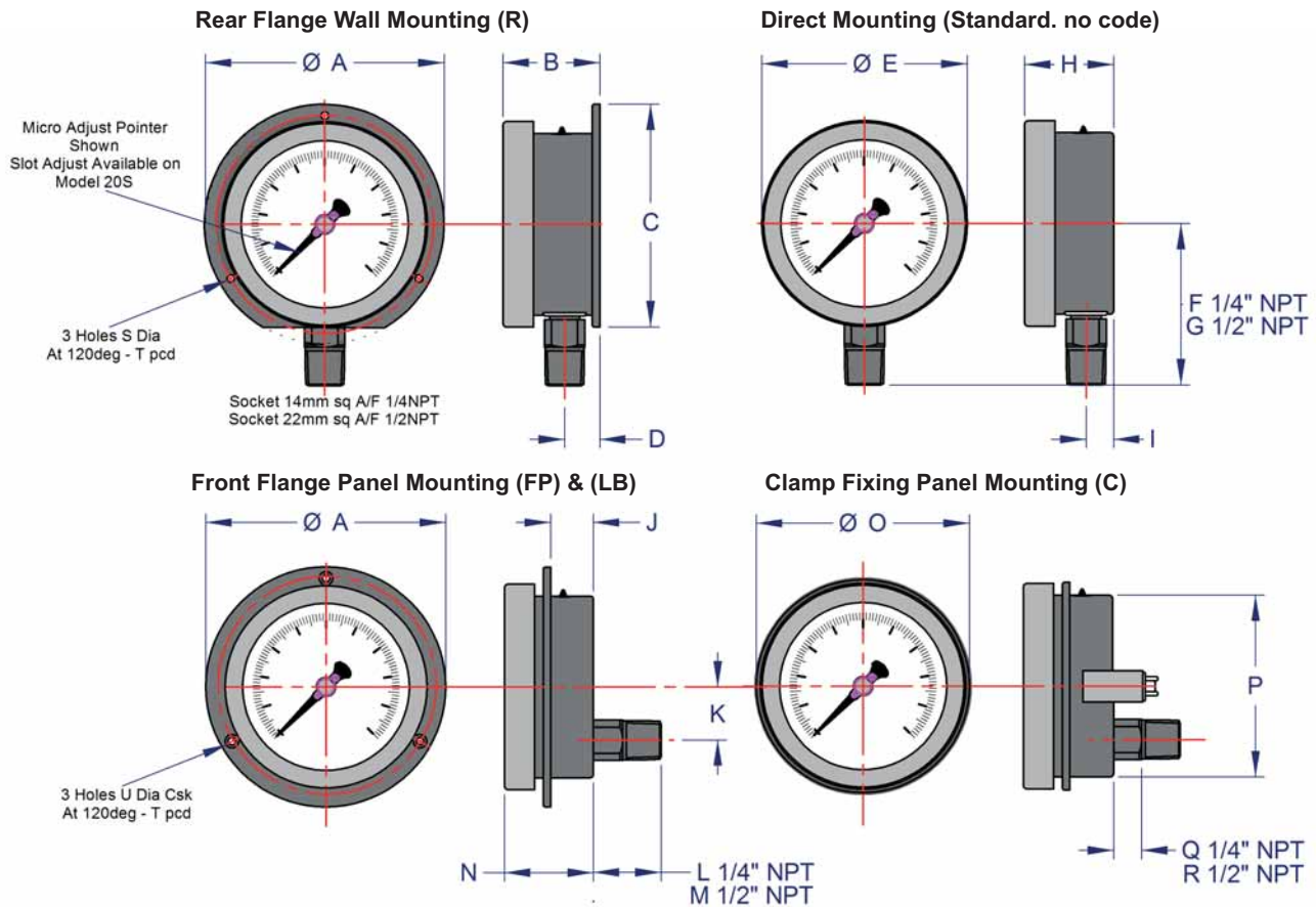
Dimension Chart (Same for VIBRAGAUGE® Option Models)
